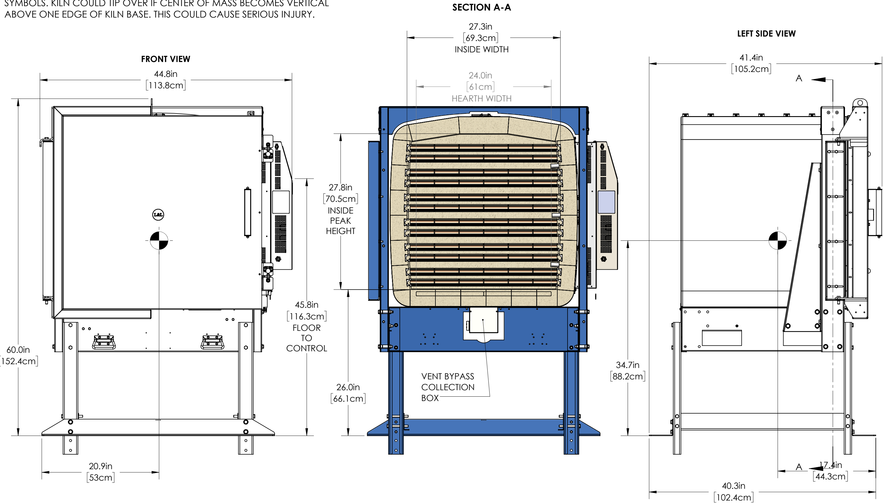
FRONT, FRONT CROSSECTION AND LEFT SIDE VIEWS
