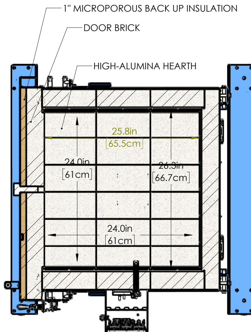
SECTION B-B TOP VIEW CUTAWAY ALL BRICK 3" THICK
