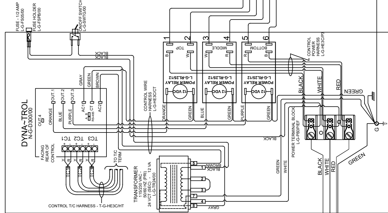
LOOKING INSIDE CONTROL PANEL
