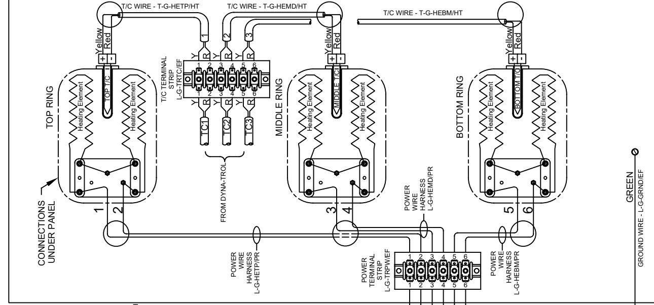
LOOKING AT OUTSIDE OF ELEMENT COVER PANEL
