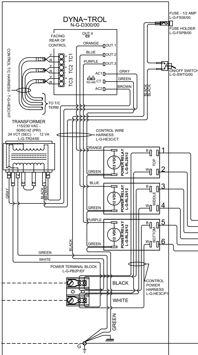
LOOKING INSIDE CONTROL PANEL
