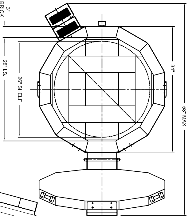
VIEW LOOKING INSIDE KILN
