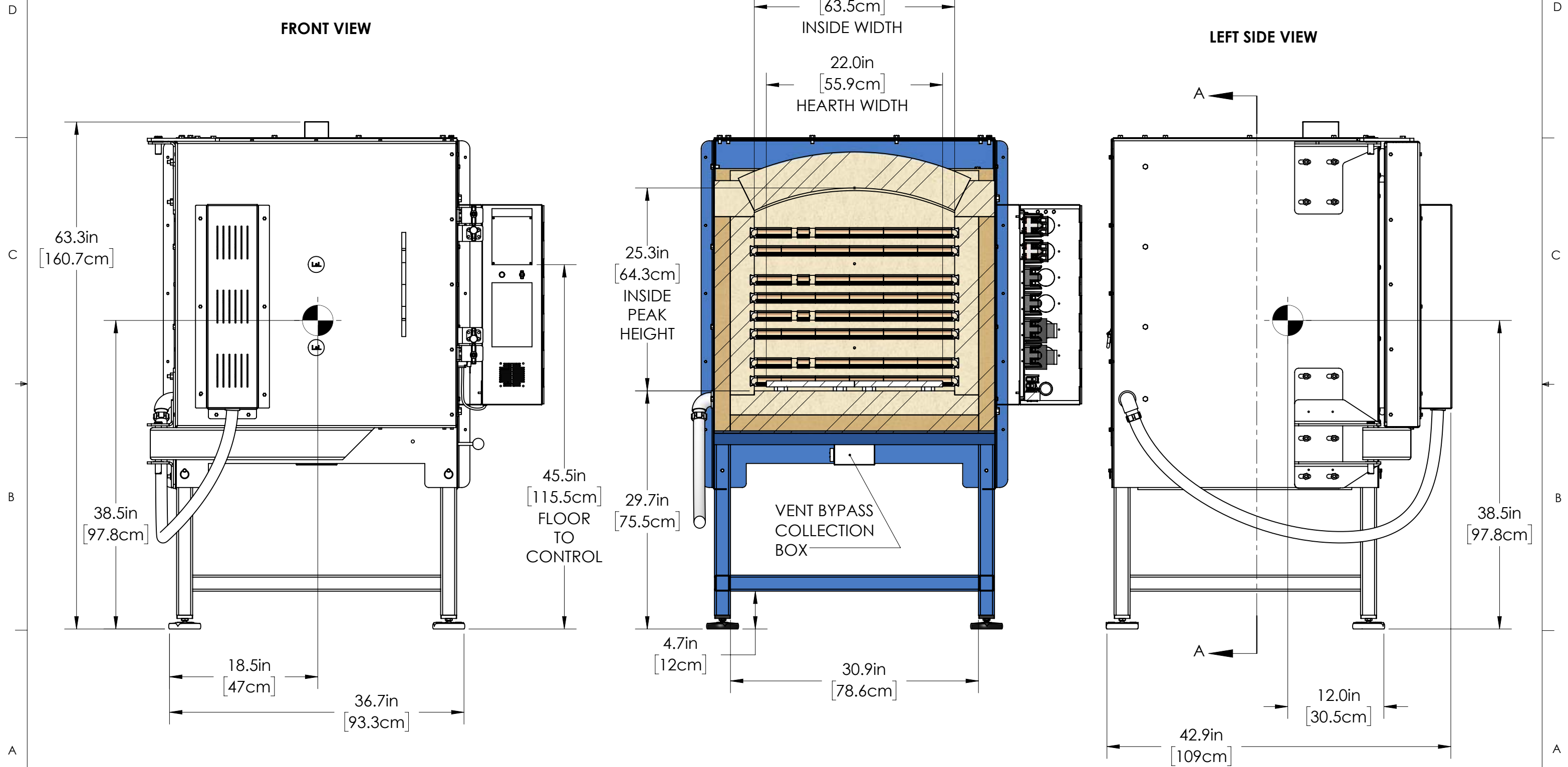
FRONT, FRONT CROSSECTION & LEFT SIDE VIEWS
